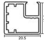
KT-71 19 mm Shutter Profile (4 mm Glass)
